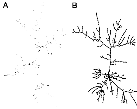
Fig. 3. Visual comparison of a real-life metabolic network with that generated by our model. (A) The backbone of the metabolic network in E. coli (8) located upstream of the central metabolism (green). (B) A similarly sized model network (red). Note the hierarchy of branch lengths in both images in which shorter pathways tend to be attached to progressively longer pathways. The branch length distributions in real and model networks are shown as green circles and red squares in Fig. 4B.
